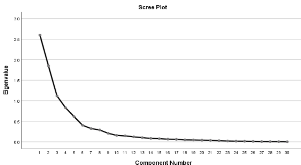
Figure 1. Scree plot
