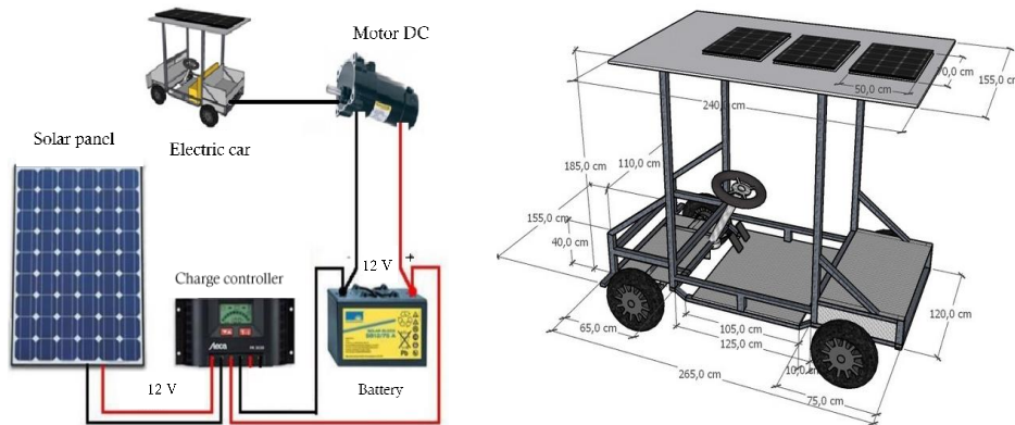
Figure 1. Scheme of solar powered electric car
